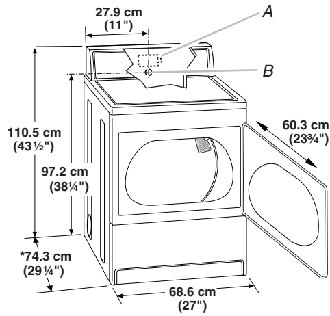
A. Terminal block cover B. Power supply cord/cable strain relief
